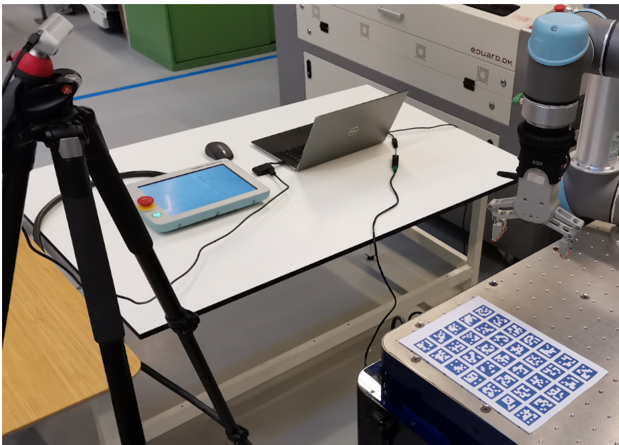
Figure C.1: Setup used for calibration, where ArUcO markers are used as an intermediate reference frame between the camera and robot.
