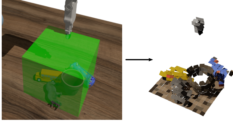
Figure 5.5: An octree that is formed from a volume of the observable workspace. In this visualisation, each finest leaf octet is represented as a square that is oriented by \bar{n} and offset from the centre of the octet by \bar{d} . Furthermore, each octet is coloured with its corresponding \overline{rgb} feature.
