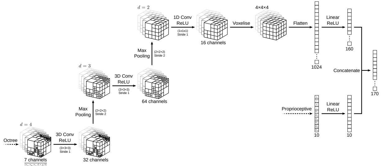
Figure 5.6: Architecture of the octree-based CNN feature extractor. Auxiliary features from proprioceptive observations are concatenated to features extracted from octrees in order to provide a single output feature vector. This network is duplicated for each of the three observation stacks and their output is concatenated into a feature vector with length of 510.
