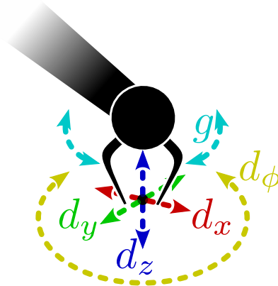
Figure 4.4: Action space of the grasping task, where (d_x, d_y, d_z) indicates a translational displacement, d_\phi is a relative yaw rotation, and the gripper closing and opening is denoted by g .
