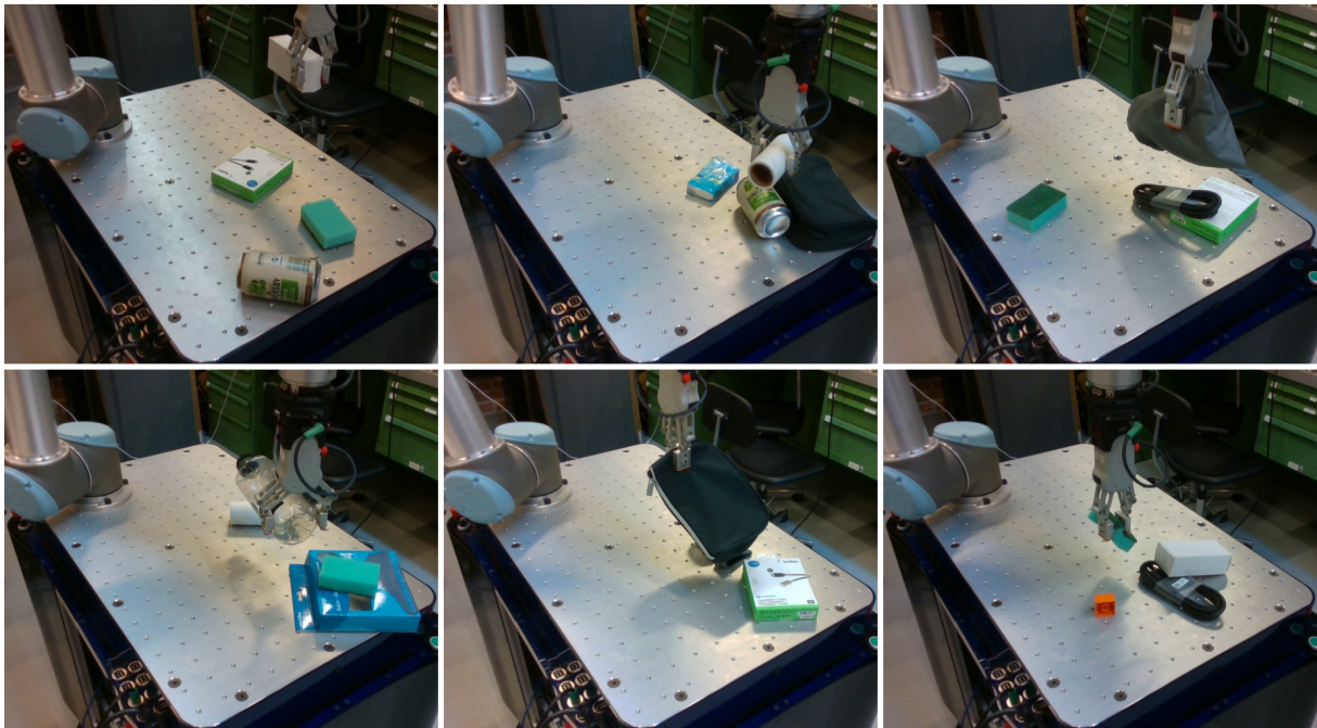
Figure 6.7: Examples of successful grasps accomplished by a policy that was transferred from simulation to real-world domain.
