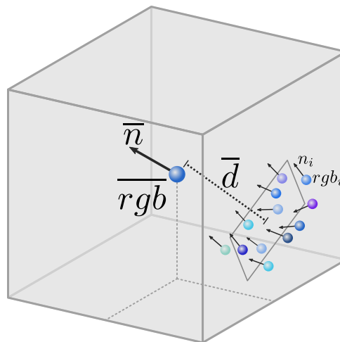
Figure 4.3: Representation of features for a single finest leaf octant from an octree. All points from the source point cloud that belong to a cell are used to determine the average unit normal vector \bar{n} , average distance to the centre of the cell \bar{d} and the average colour \overline{rgb} .
