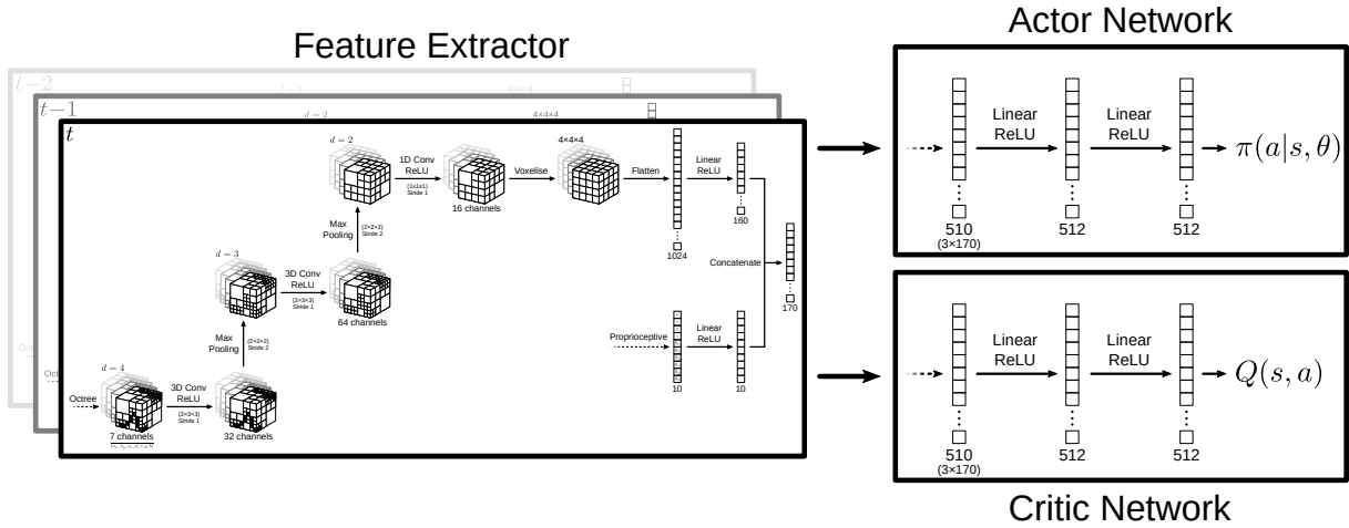
Figure 5.7: Network architecture that is used in this work for all utilised actor-critic algorithms. The feature extractor from Figure 5.6 is duplicated for each stack in order to process two historical observations in addition to the current one.
