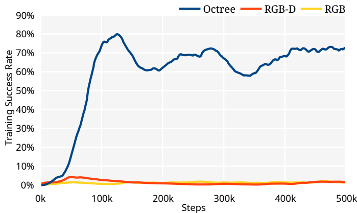
Figure 6.4 & Table 6.3: Results of octree-based, RGB and RGB-D feature extractors on the full environment that randomises camera pose on each episode.
