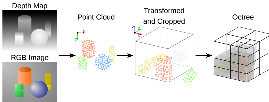
Figure 4.2: Process of constructing an octree from depth map and RGB image via an intermediate point cloud, which is transformed into the robot coordinate frame and cropped to a fixed volume.
