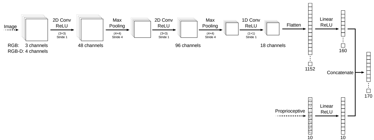
Figure E.1: Feature extractor used for RGB and RGB-D observation during experimental evaluation.
