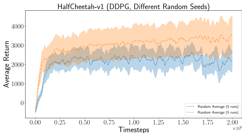
Figure 2.4: Learning curve of DDPG on a locomotion environment for two sets of five different random seeds. All runs use the same hyperparameter configuration. (Henderson et al., 2018)
