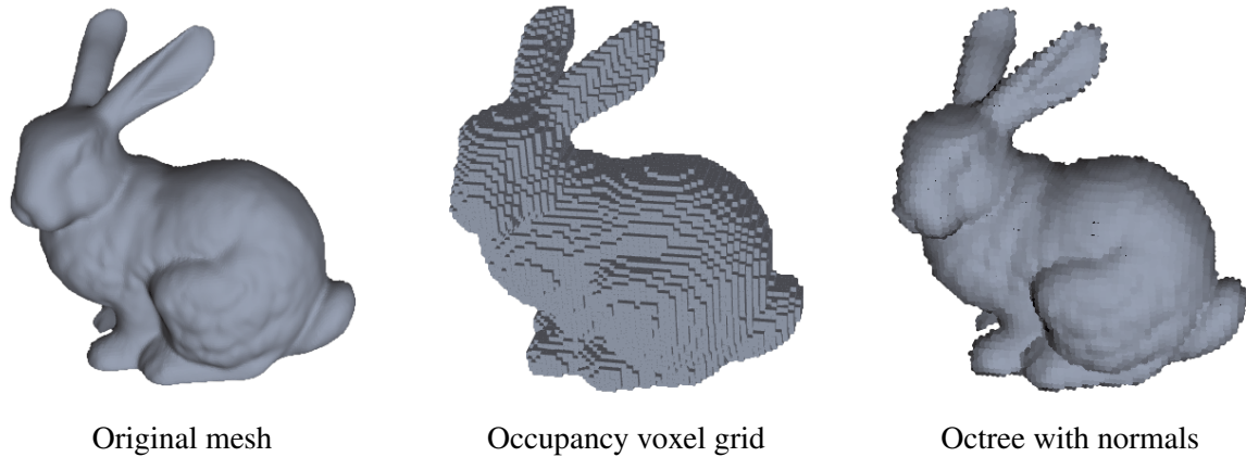
Figure 2.9: Comparison between occupancy voxel grid and smoothness-preserving octree that uses normal vector instead of binary indicator. Octree is rendered with oriented disks sampled at the finest leaf octants. Smallest cell size is the same for both representations. (Wang et al., 2017)
