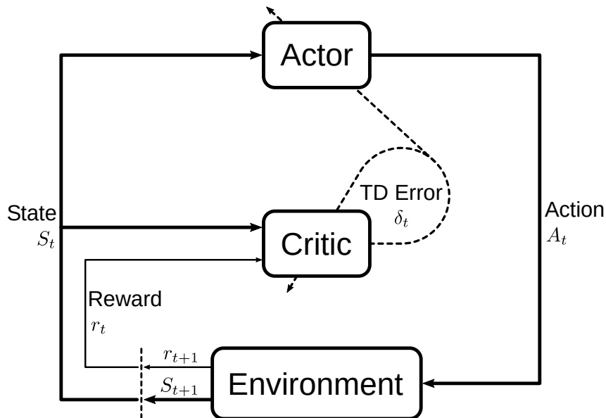
Figure 3.2: Overview of actor-critic methods. TD error \delta_t is used to adjust both critic’s action-value function Q(s, a) and actor’s policy \pi(a|s, \theta) . Adapted from Sutton and Barto (2018).
