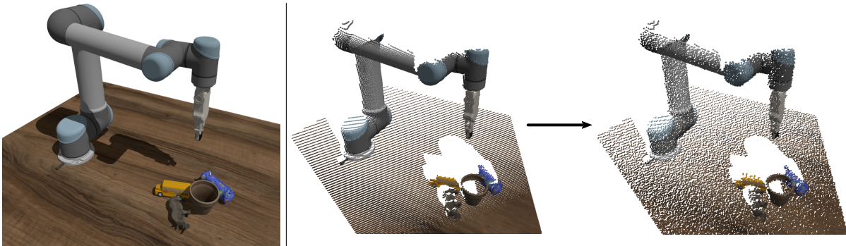
Figure 5.2: Effect of adding Gaussian noise to RGB-D data in order to improve resemblance to noise of real-world camera sensors.
