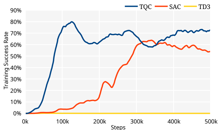
Figure 6.3 & Table 6.1: Comparison of TQC, SAC and TD3 algorithms on the created grasping environment. The training success rate is processed with a moving average, n = 100 , and exponential smoothing, \alpha = 0.002 , for all agents.
