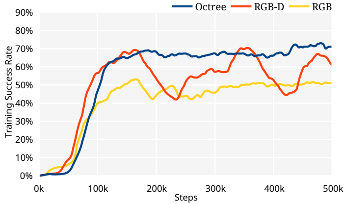
Figure 6.5 & Table 6.4: Results of octree-based, RGB and RGB-D feature extractors on environment with a fixed camera pose.
