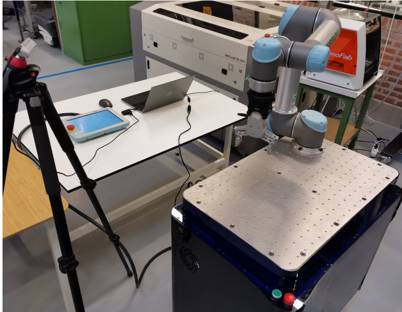
Figure 6.1: UR5 robot with RG2 gripper and RealSense D435 camera in a setup that is used to evaluate sim-to-real transfer.
